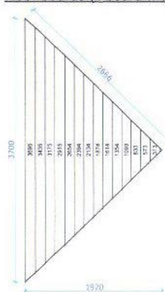
Roof boards (if board width is 135mm)
