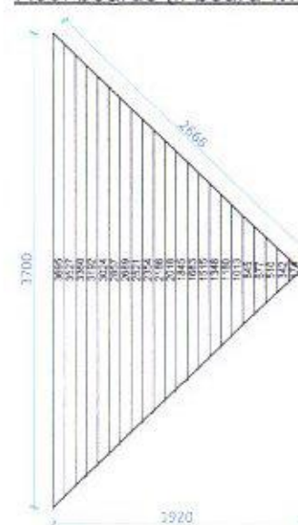
Roof boards (if board width is 87mm)
