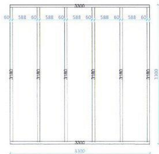
Floor bearers 1:50
