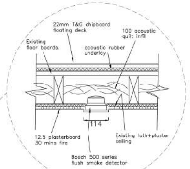
Flush Smoke Detector Detail A3 = 1:10
