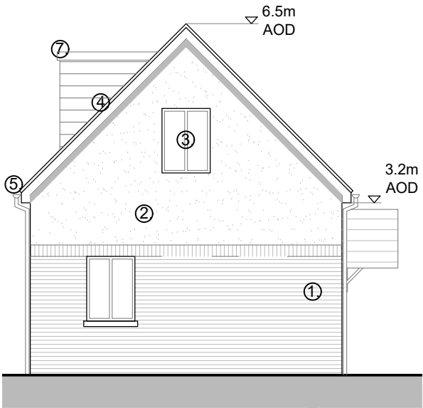
WEST ELEVATION
