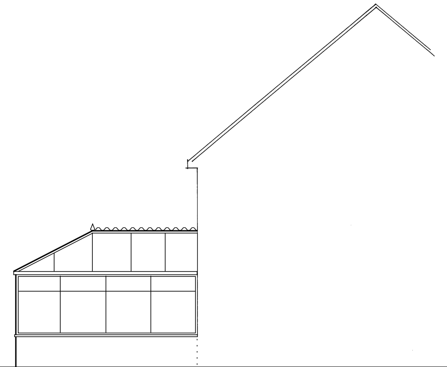
Proposed South/Side Elevation
