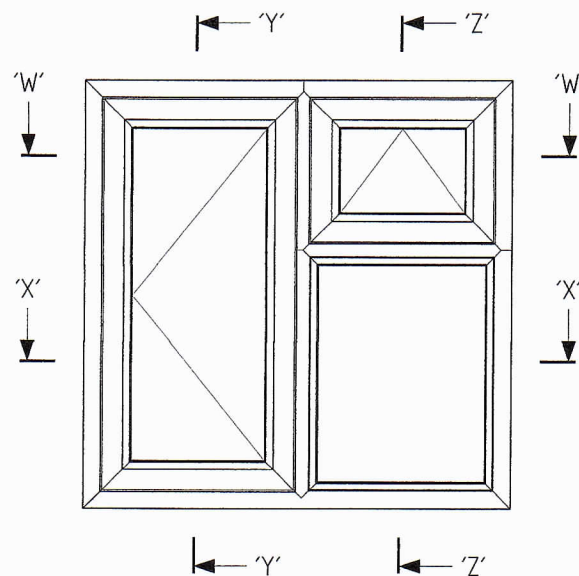
Typical Elevation (Viewed from outside) Scale 1:20
