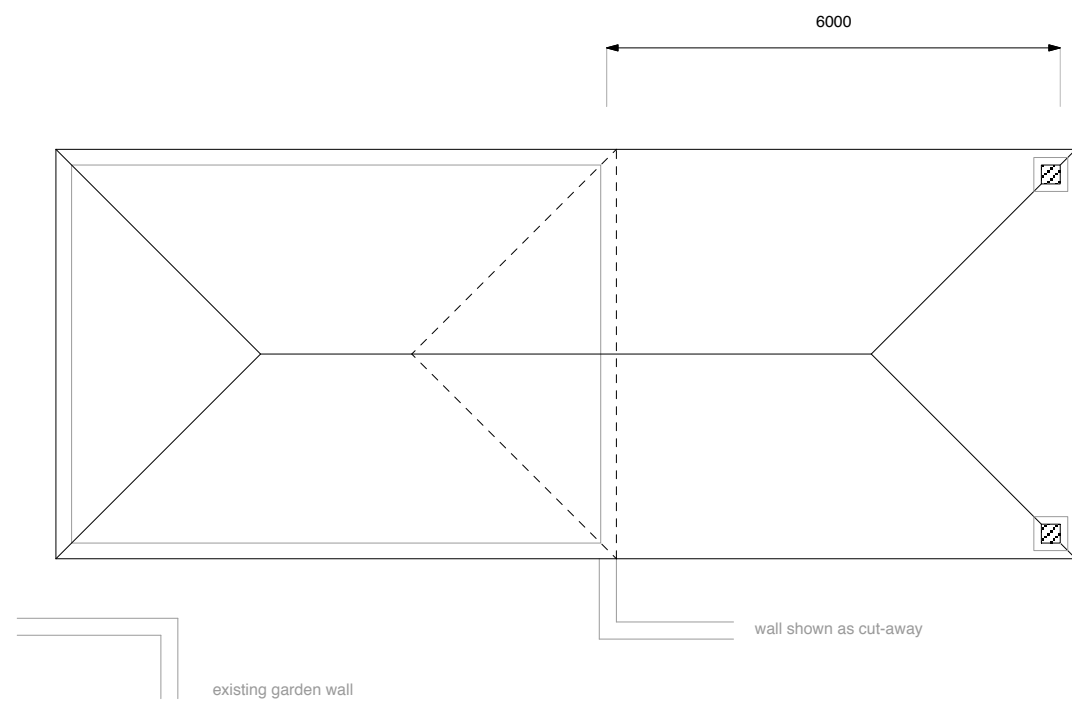
Proposed Roof Plan at 1:100 scale
