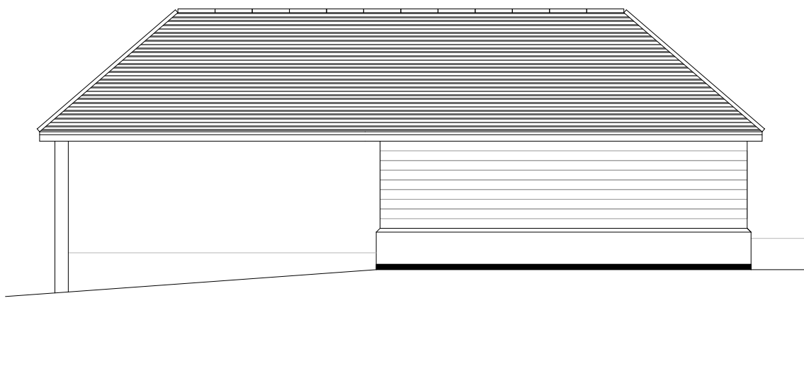
Proposed SOUTH WEST (Rear) Elevation at 1:100 scale
