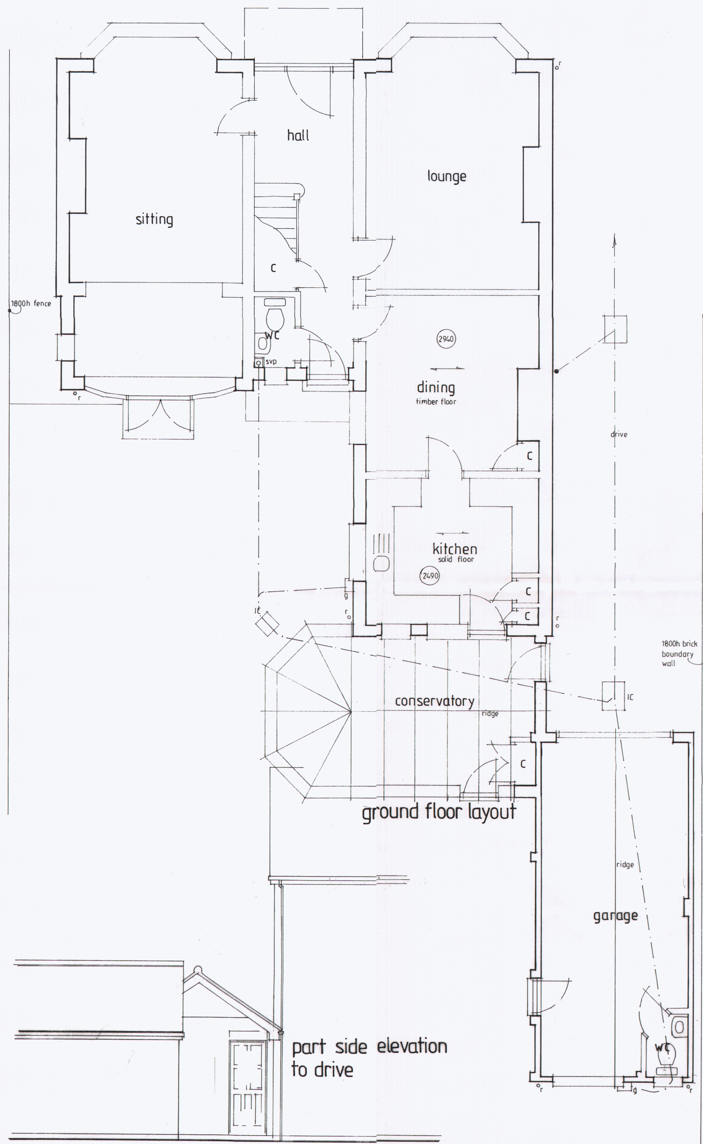
EXISTING SURVEY, 43 LANGSTONE ROAD, HAVANT, PO9 1RB.
