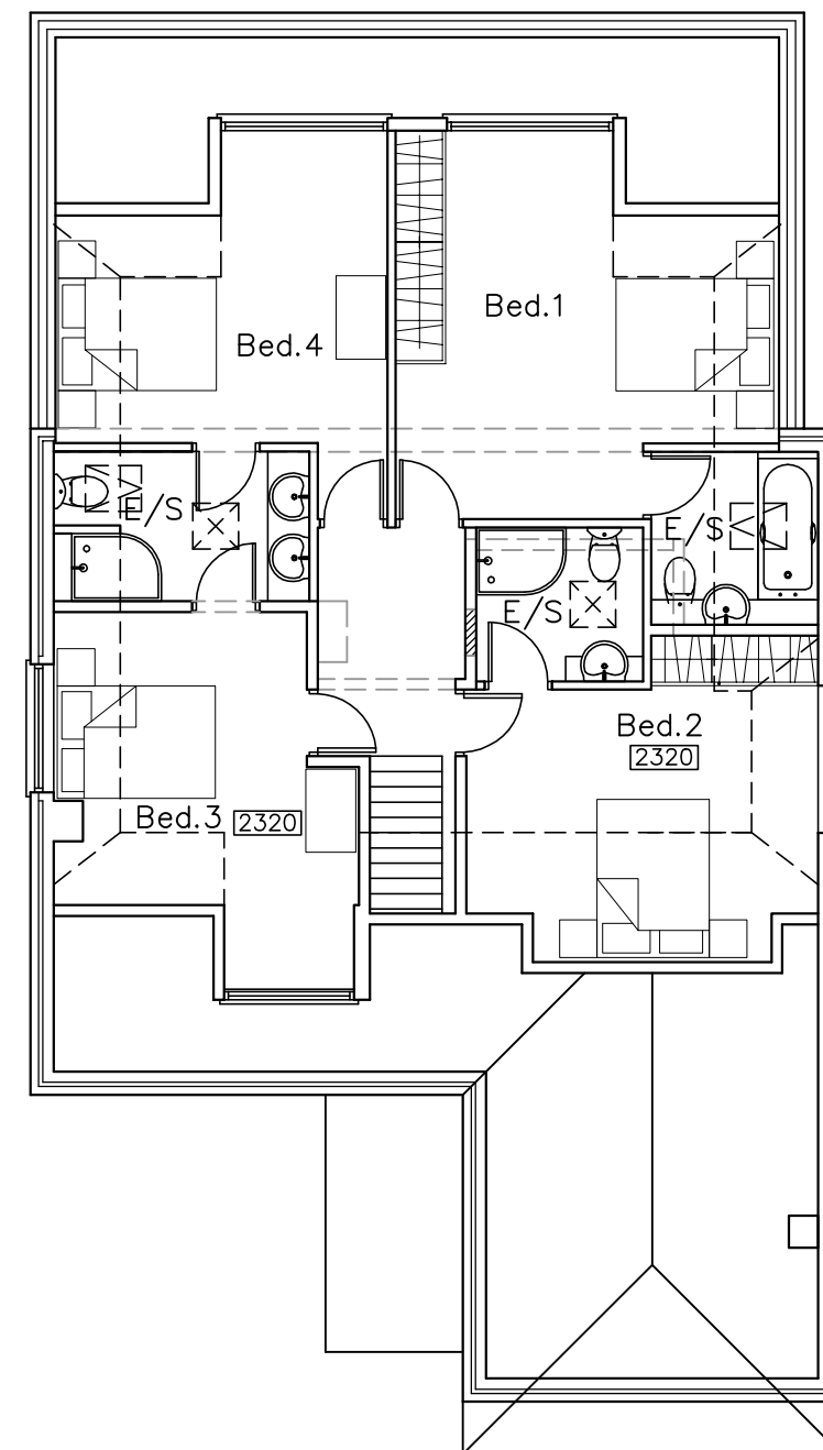
FIRST/LOFT
