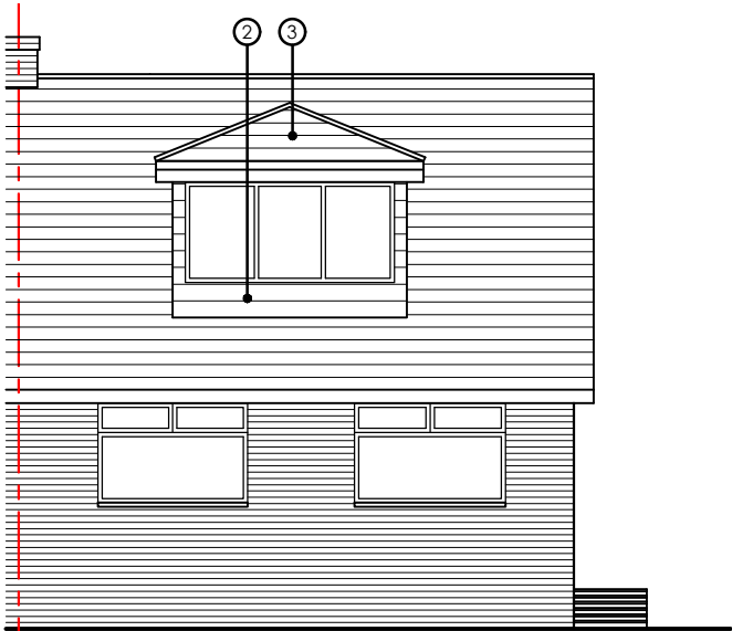
PROPOSED SOUTH ELEVATION OPTION 1
