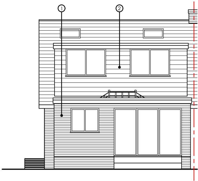
PROPOSED NORTH ELEVATION OPTION 1
