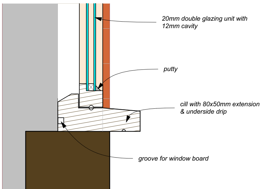
Casement opening 1:5
