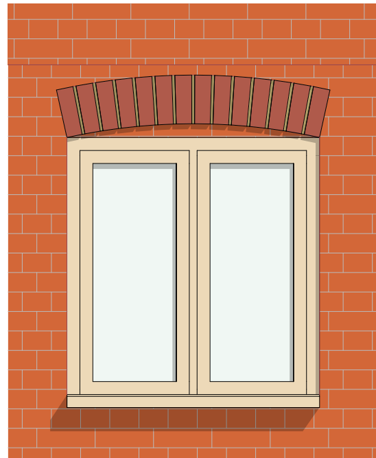
Casement opening 1:20
