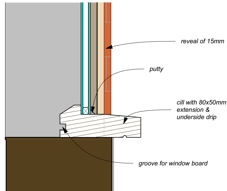
Hayloft opening 1:5
