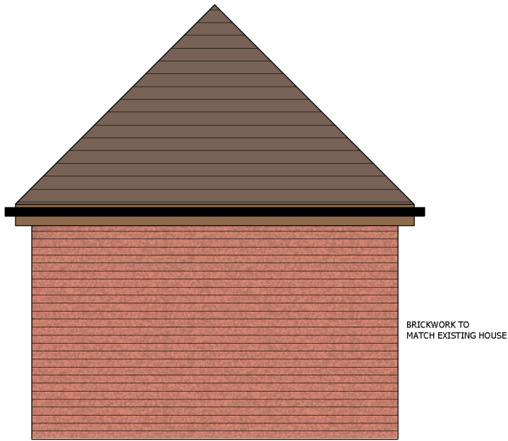
SOUTH ELEVATION
