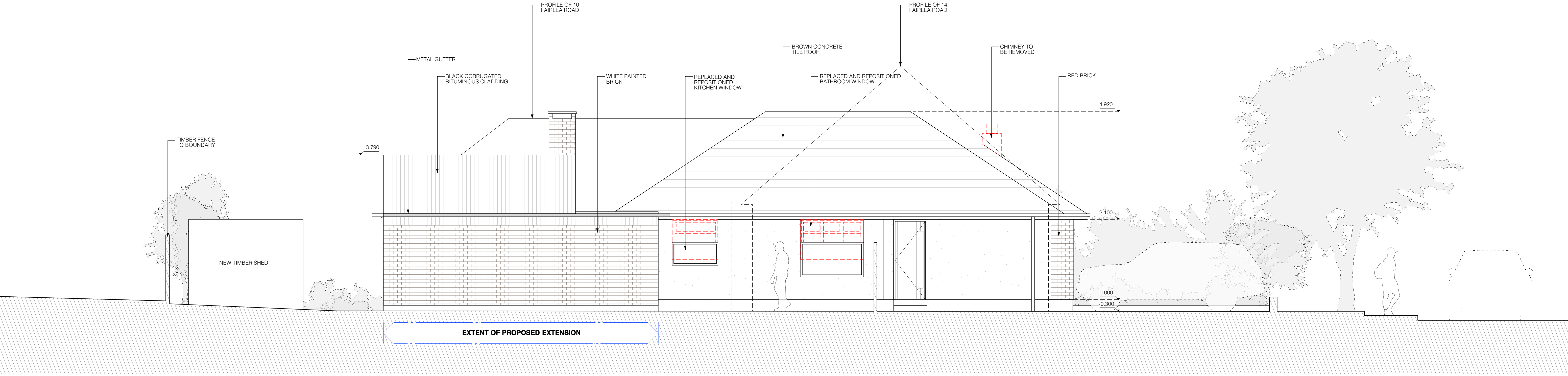
01 PROPOSED WESTERN ELEVATION 1:50
