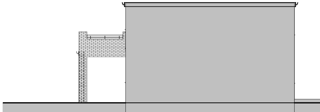
3 East Elevation 40 1 : 100
