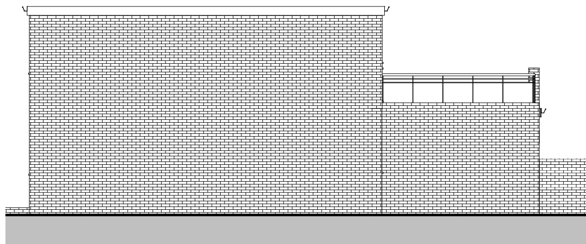
4 West Elevation 40 1 : 100
