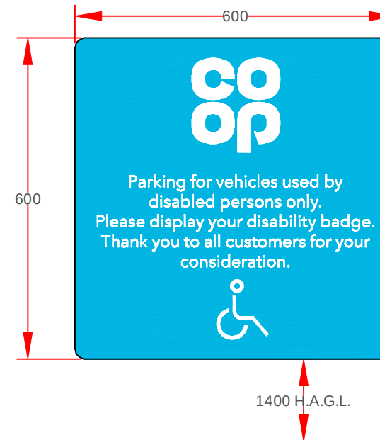
Sign I - Scale 1:10
