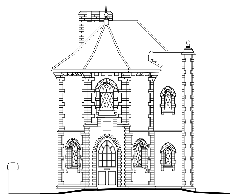
North Elevation
