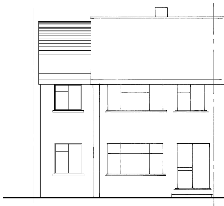
Proposed South/Front Elevation
