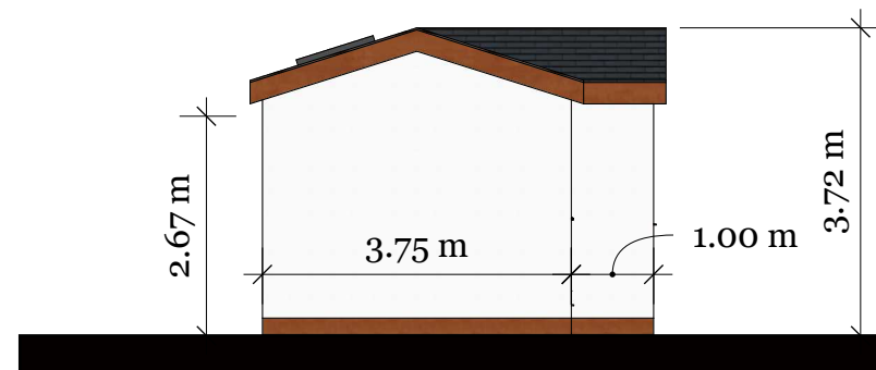
South Elevation
