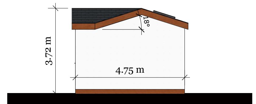
East Elevation
