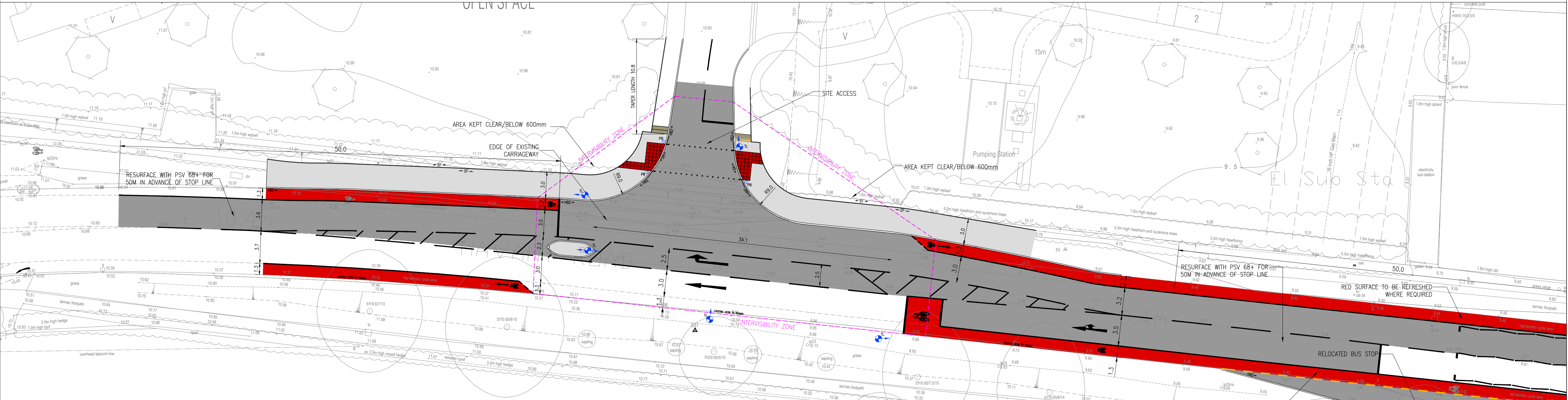
SIGNAL JUNCTION (SCALE 1:250)
