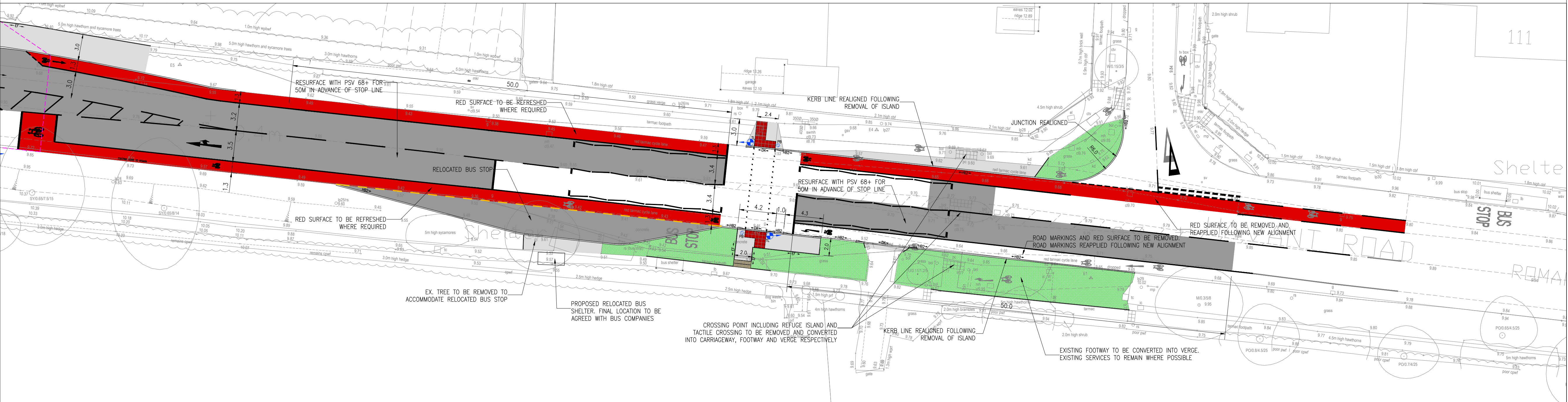
PEDESTRIAN CROSSING ARRANGEMENT (SCALE 1:250)
