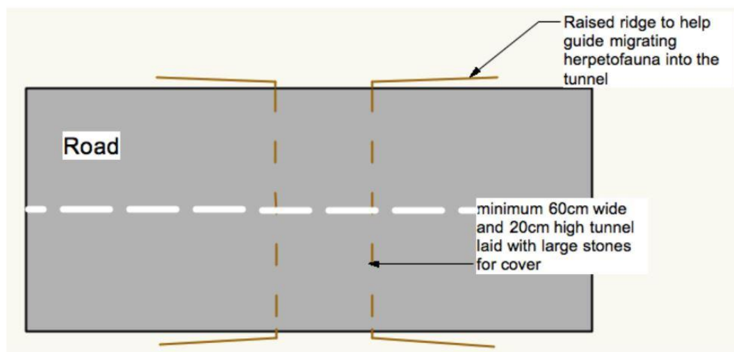
Figure 7: An amphibian tunnel will connect the pond and the wetland habitats
