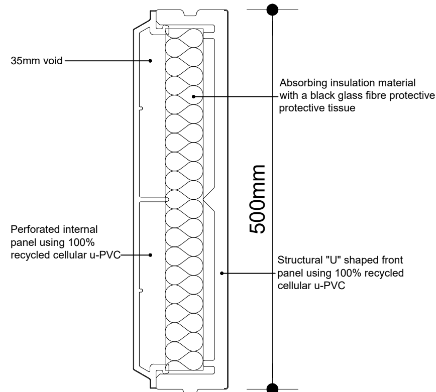
PLAN OF FENCING PANELS
