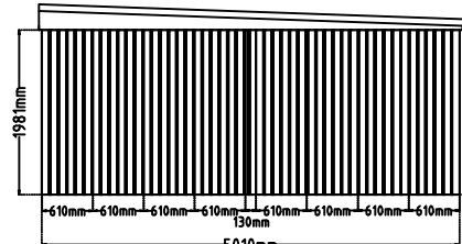
Side elevation
