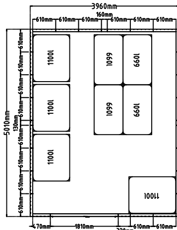
Plan view
