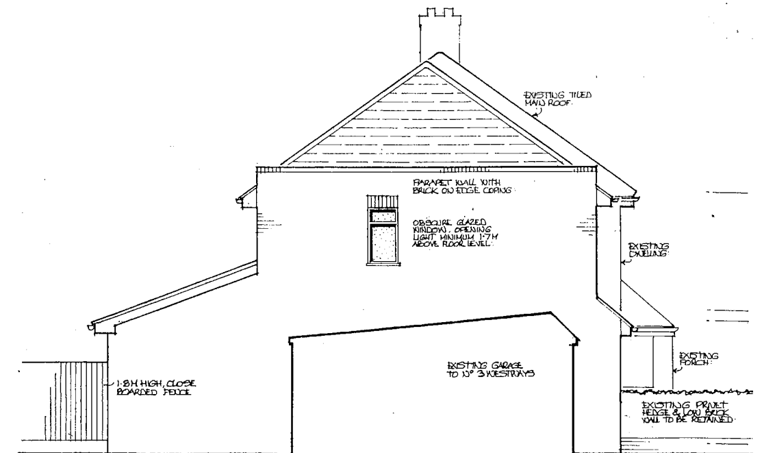
North Elevation
