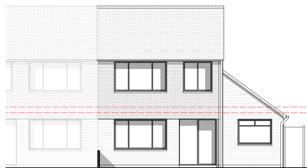
West Elevation (Existing) 1:100
