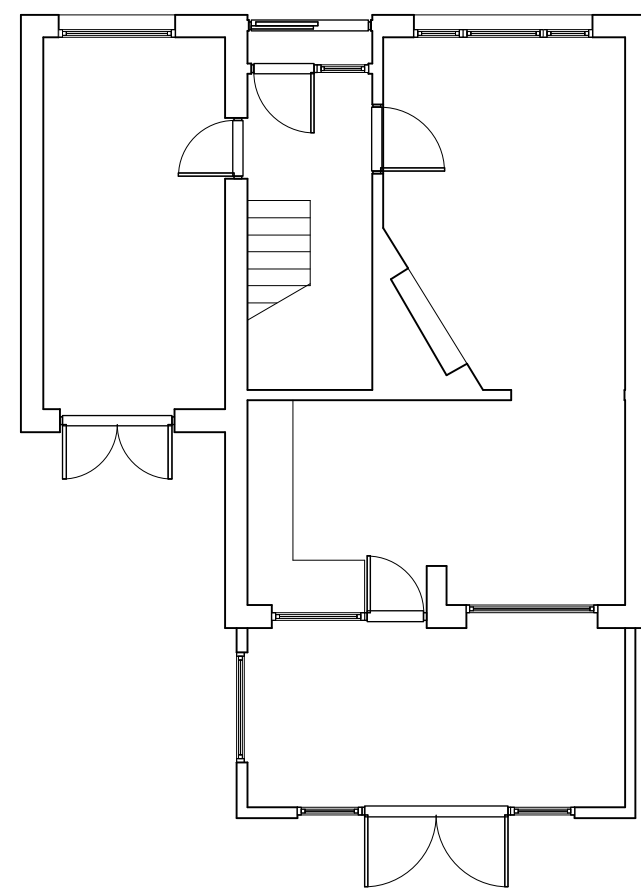
Ground Floor Plan (Existing) 1:100
