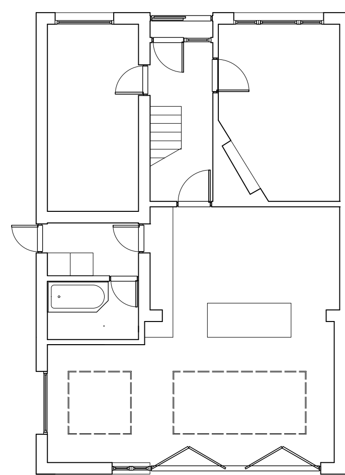
Ground Floor Plan (Proposed) 1:100
