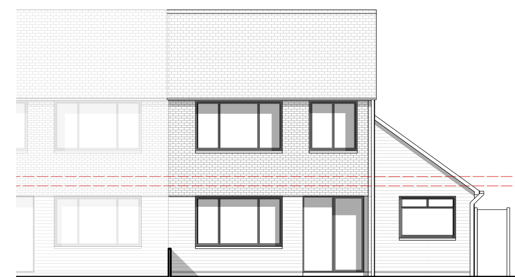
West Elevation (Proposed) 1:100
