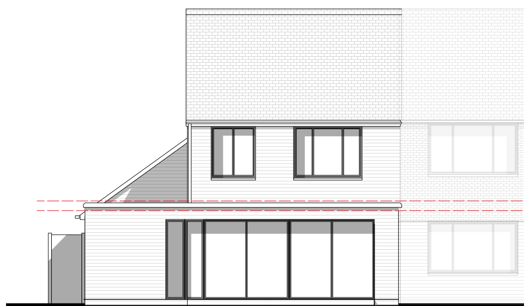
East Elevation (Proposed) 1:100
