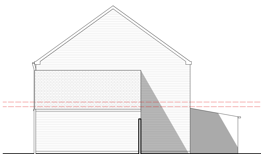
South Elevation (Existing) 1:100
