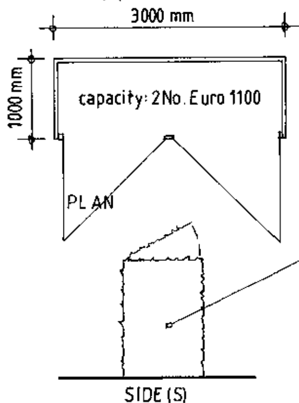
BIN STORE
