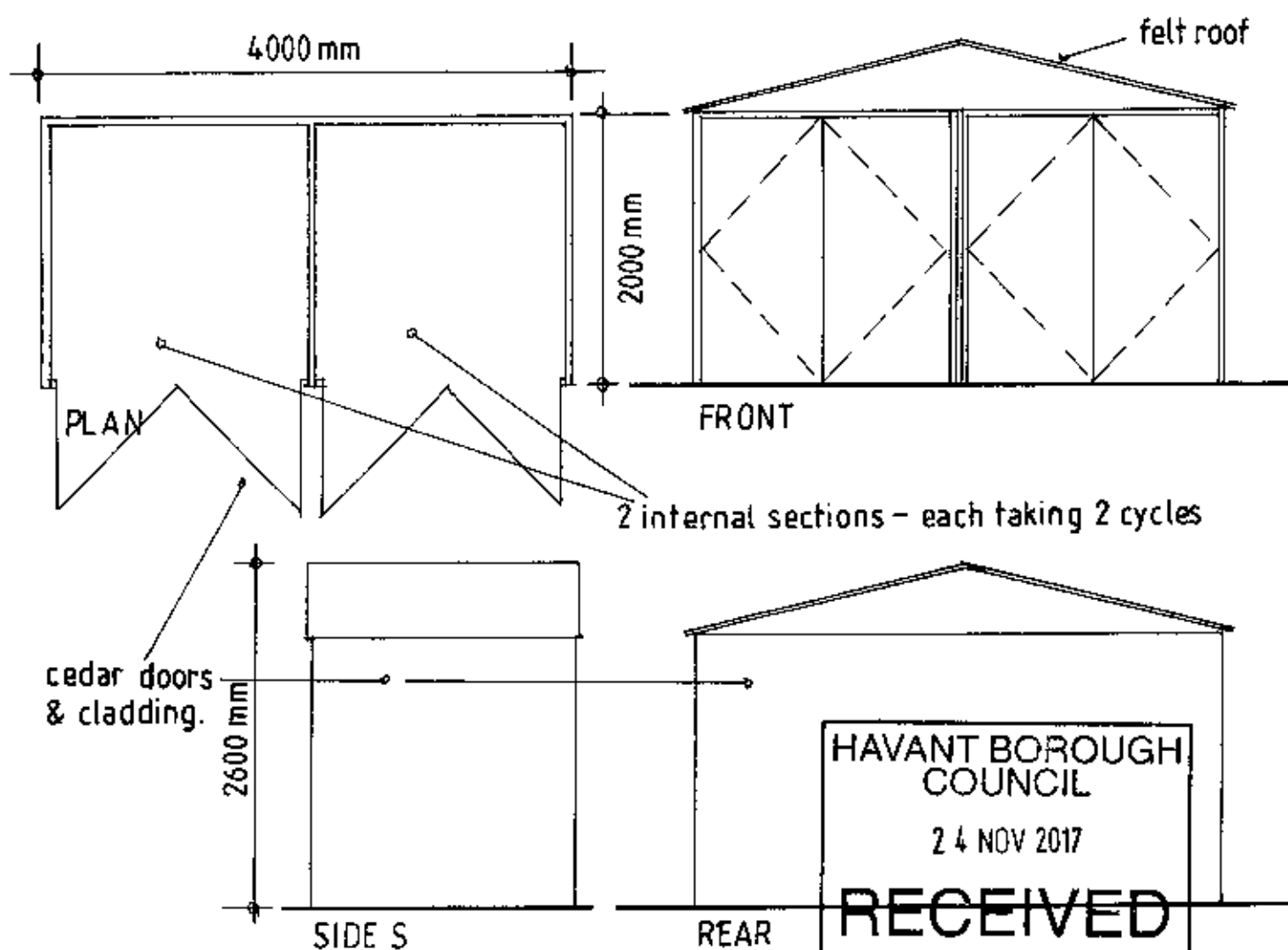
CYCLE STORE
