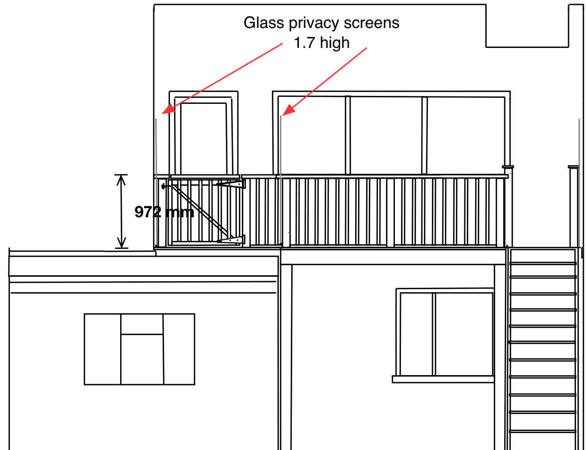
Rear Elevation 1:50
