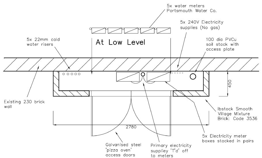
Chimney Plan Section
