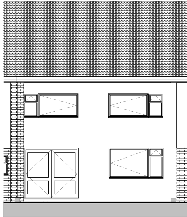
1 North Elevation 40A 1 : 100
