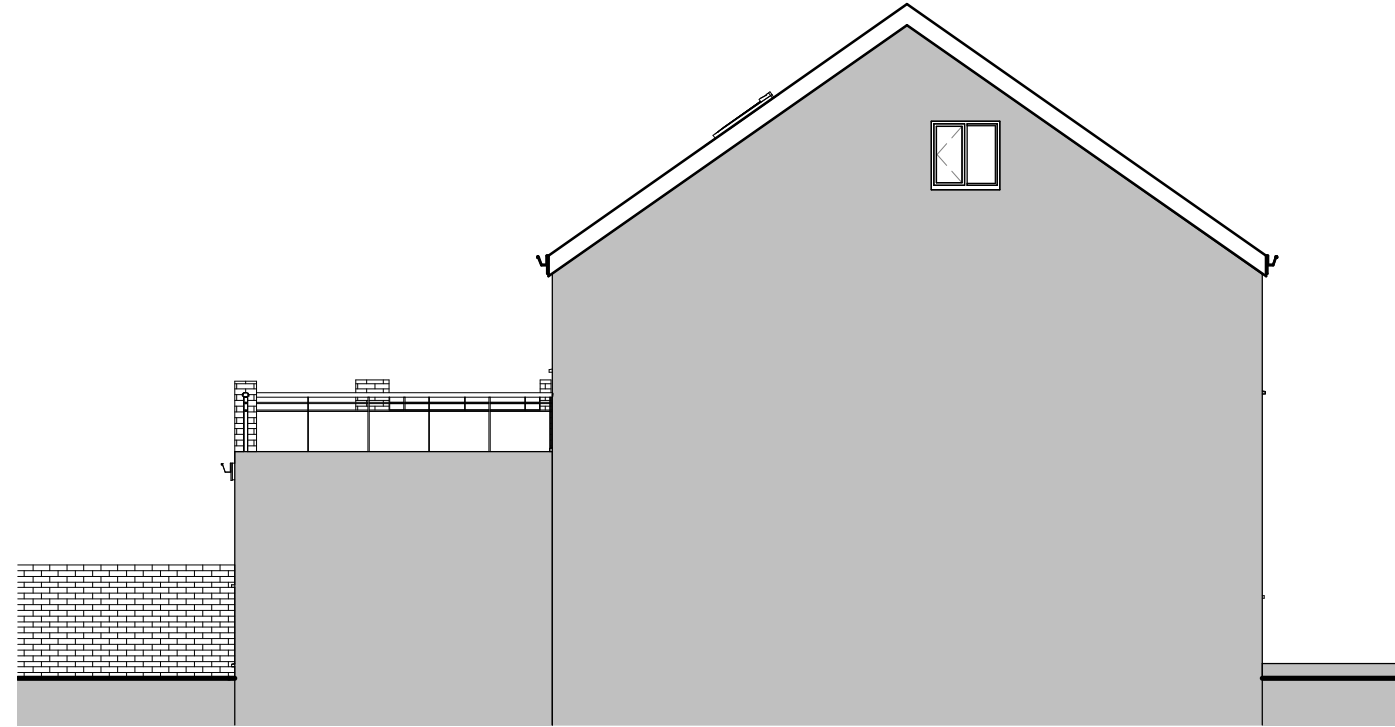
3 East Elevation 40 A 1 : 100
