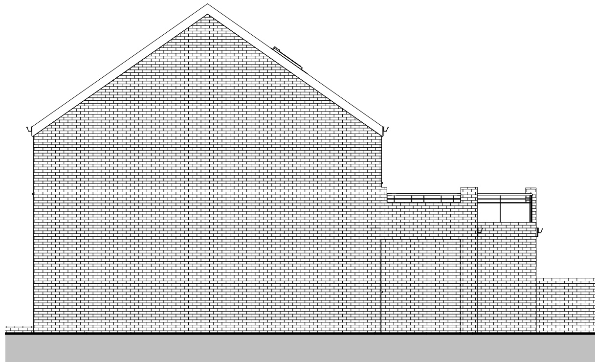
4 West Elevation 40 A 1 : 100
