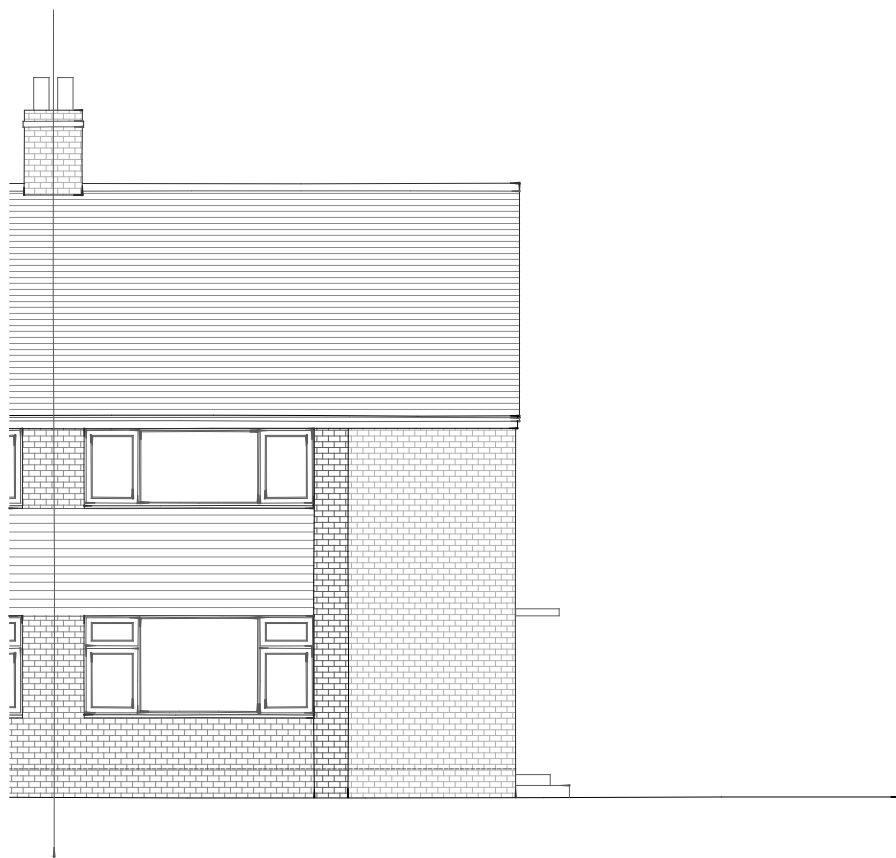
South-East (Front) Elevation - As Existing
