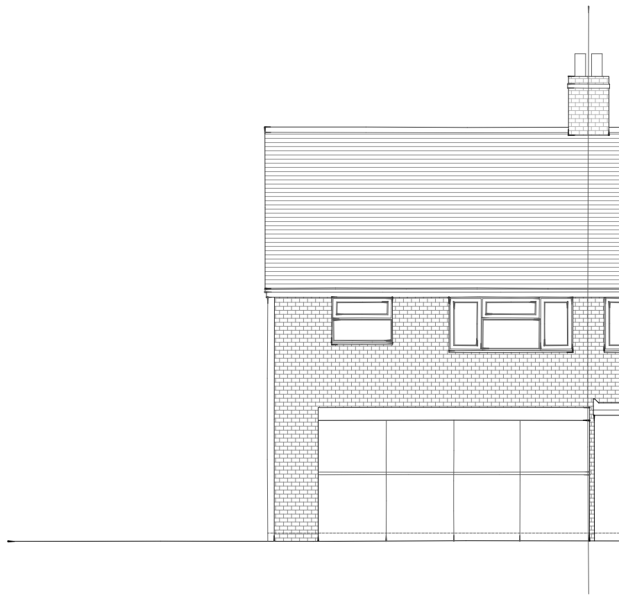
North-West (Rear) Elevation - As Existing
