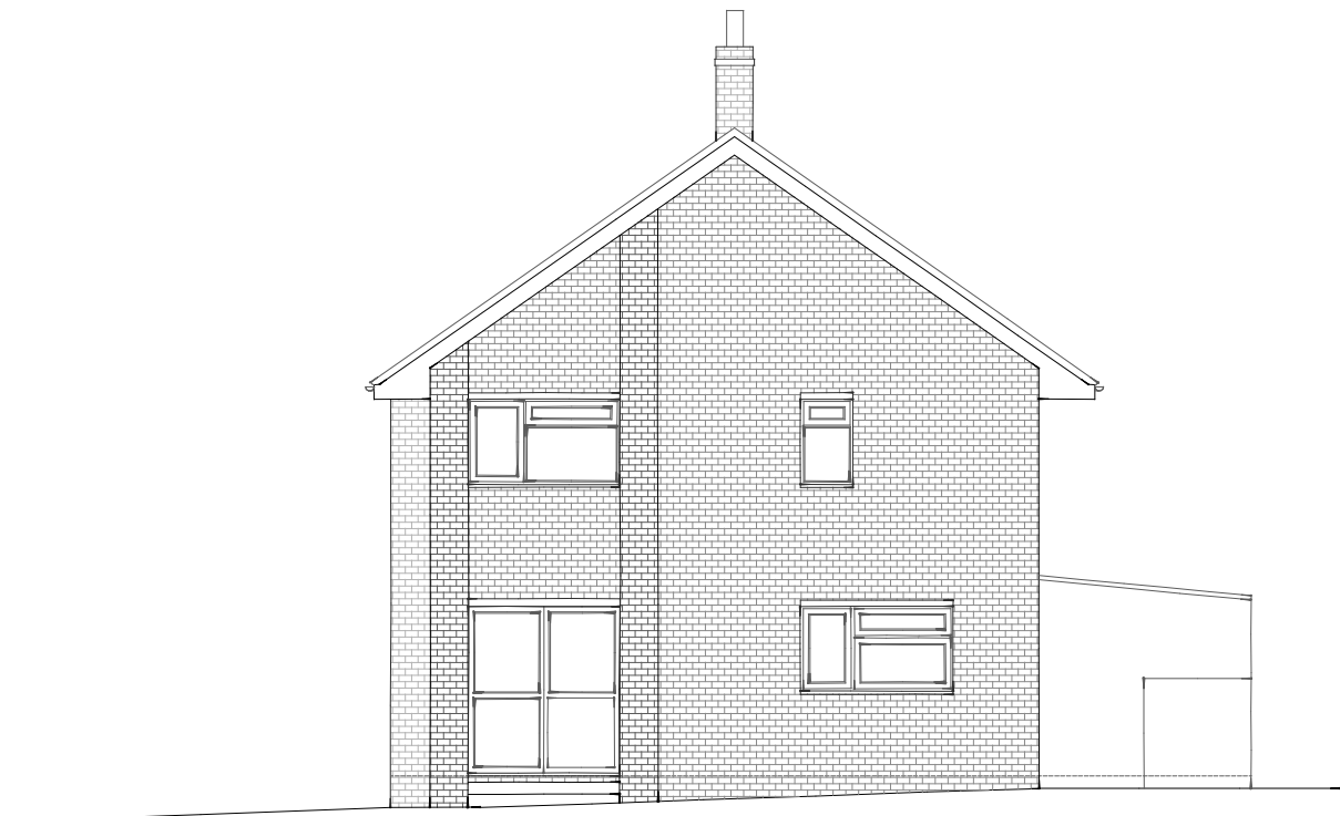
North-East (Side) Elevation - As Existing
