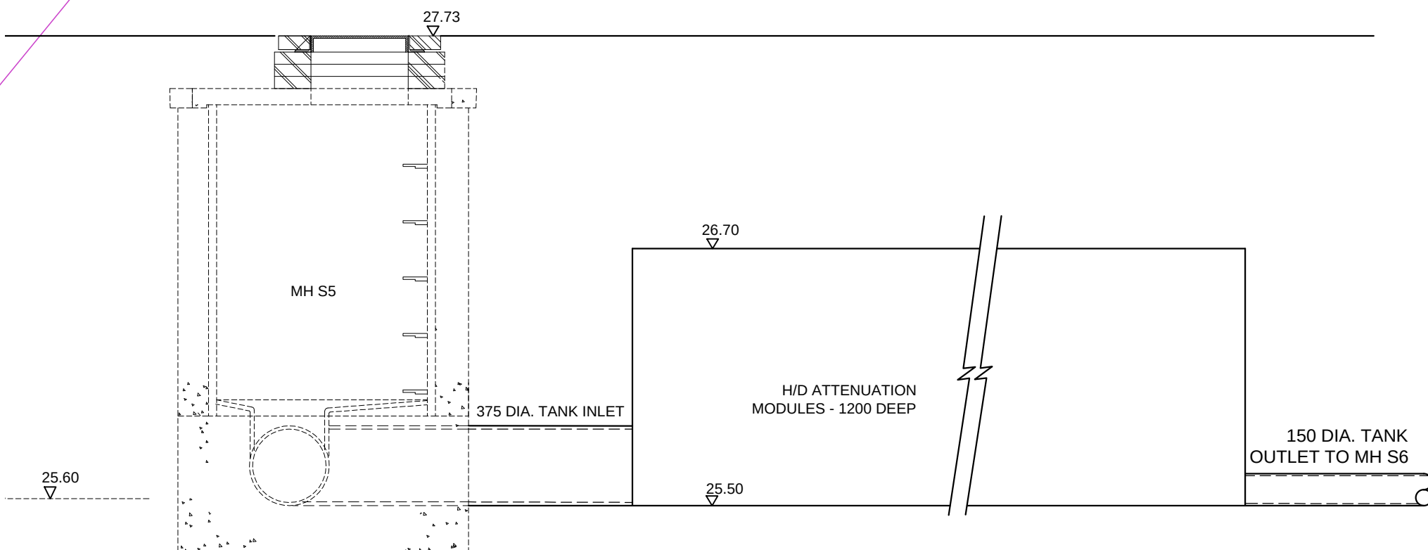
ATTENUATION TANK INLET FOR MH S5 (1:25)
