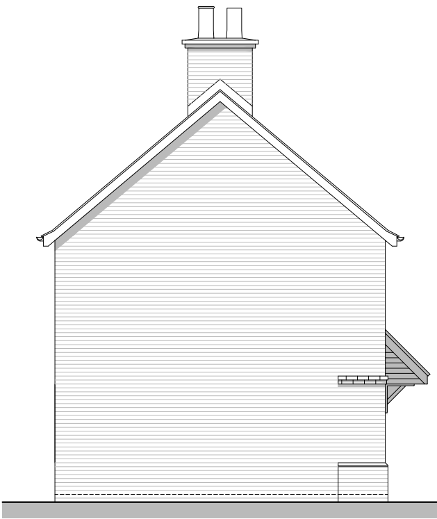
Side Elevation A
