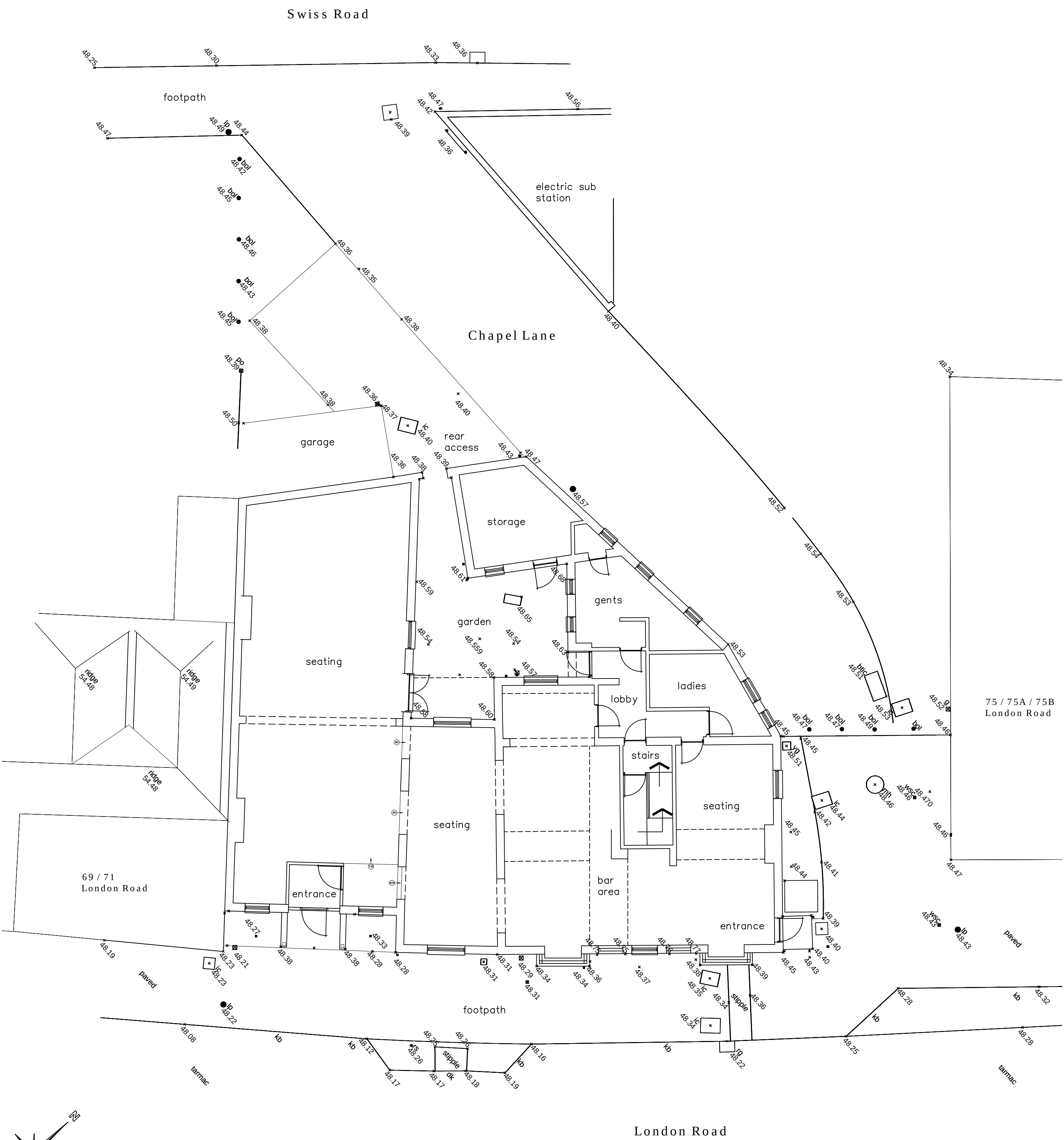
EXISTING GROUND FLOOR / SITE LAYOUT SCALE 1:100
