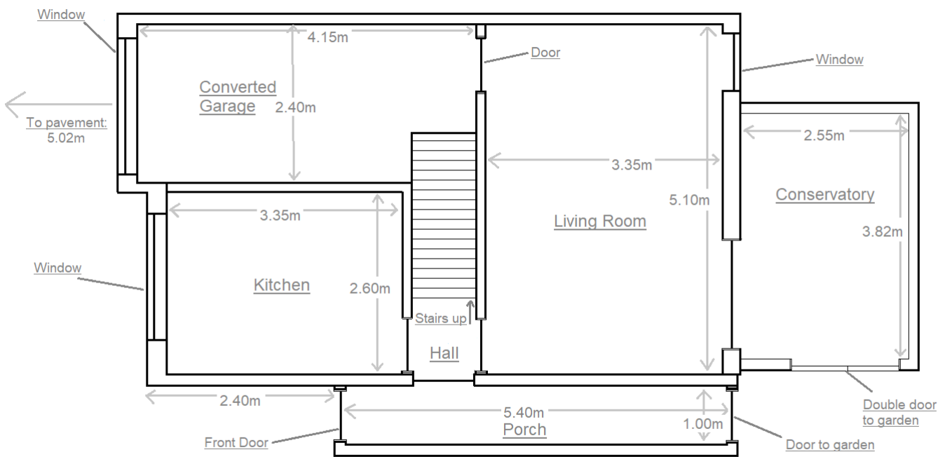
6 Mountbatten Drive Ground Floor Plan - Proposed
