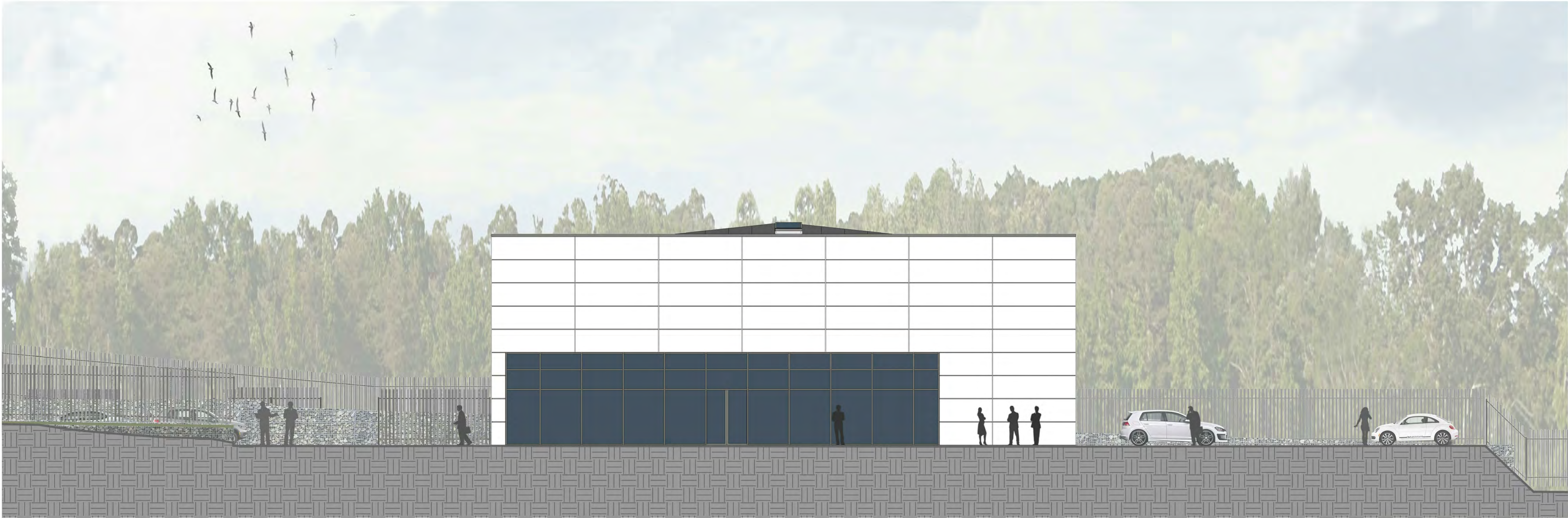
West Elevation 1:100
