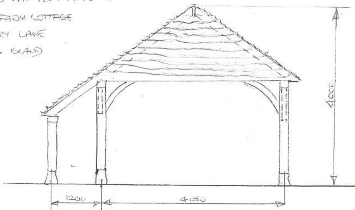
ELEVATION TO CAR PORT AA
