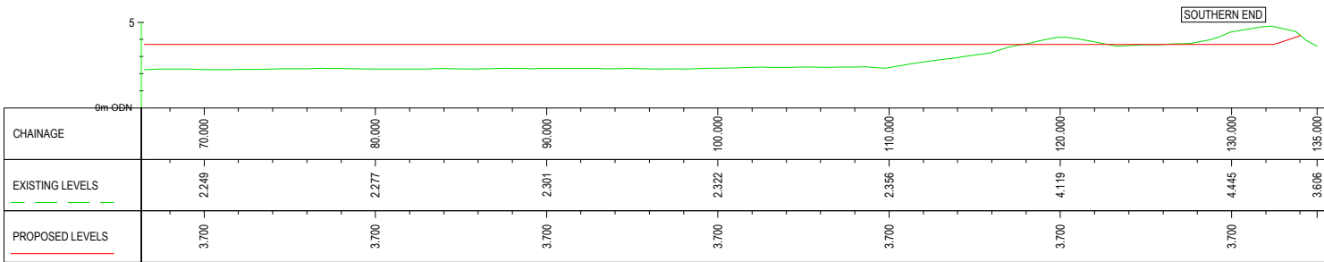
EAST MILL LANE EMBANKMENT LONG SECTION H 1:200,V 1:200
