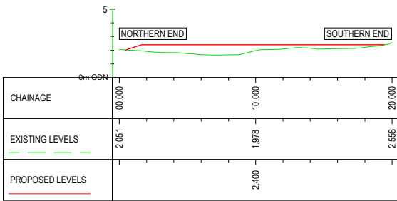
RAISED ASSET EMBANKMENT LONG SECTION H 1:200,V 1:200
