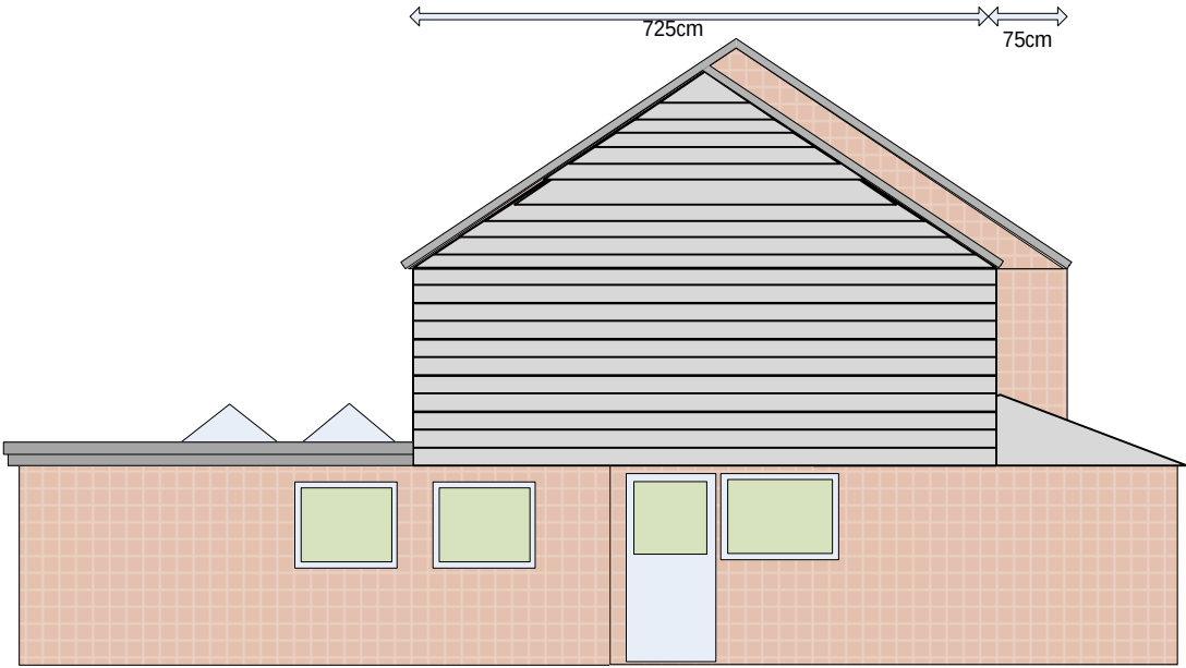
Left Elevation Proposed
