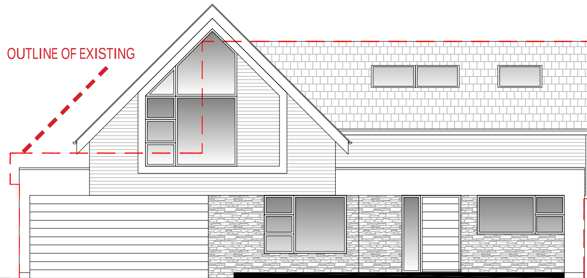
South East Elevation | Proposed
