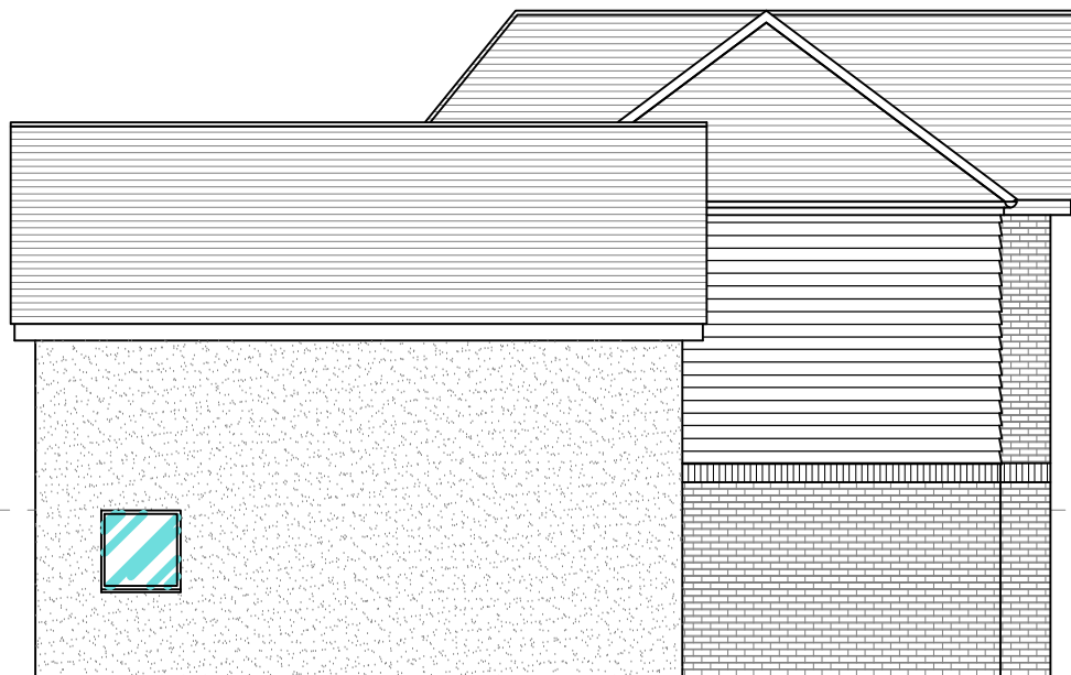
EXISTING NORTHEAST SIDE ELEVATION
