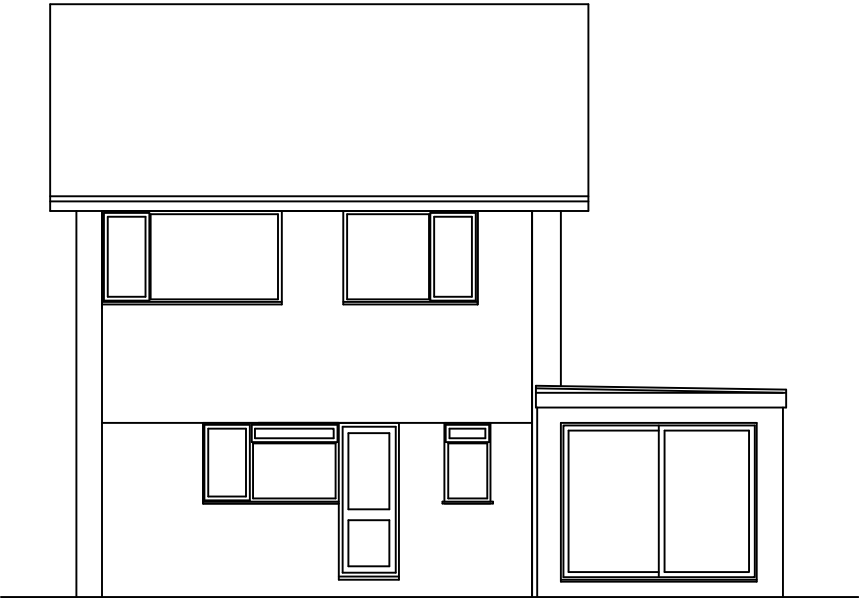
WEST ELEVATION
