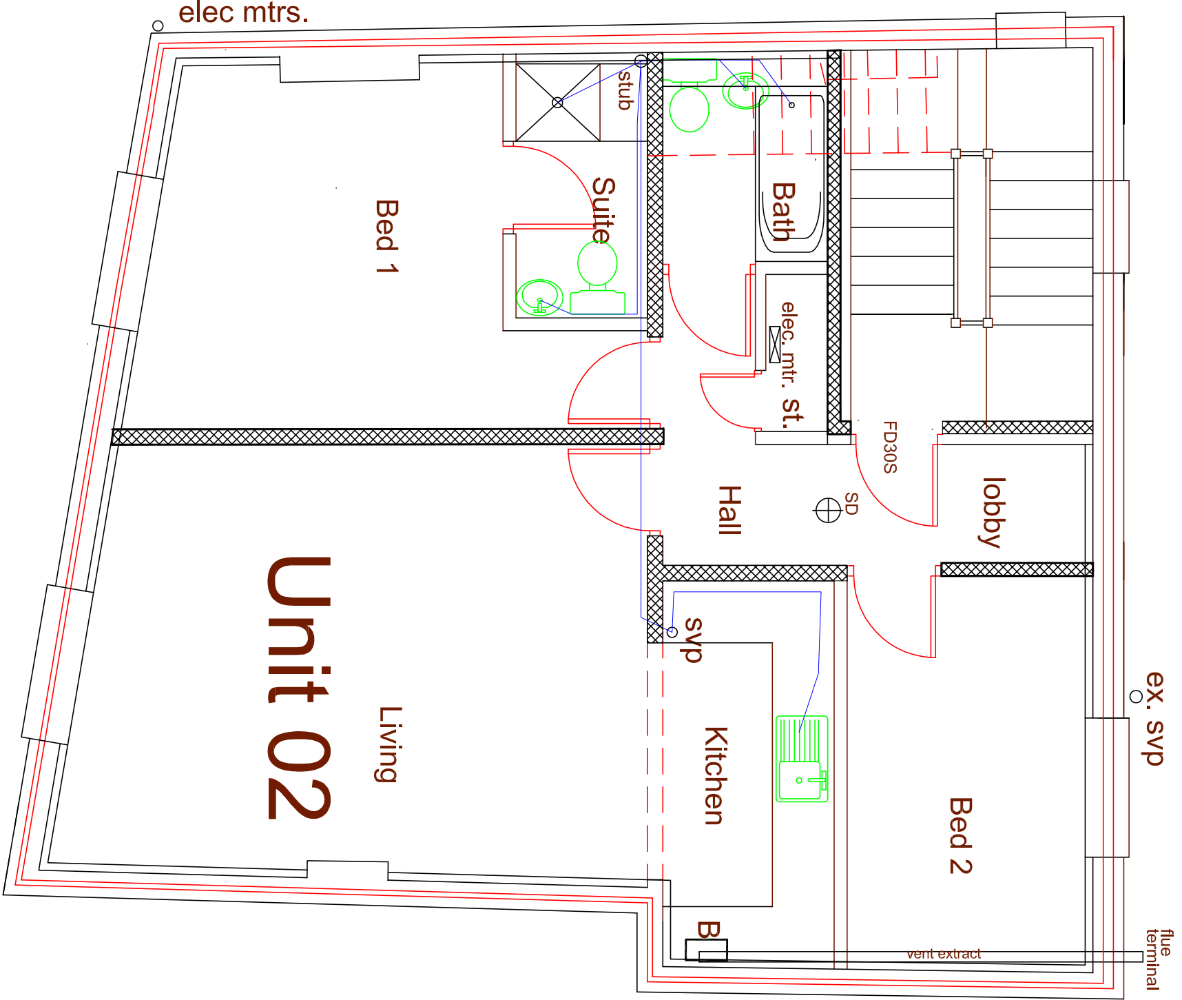
FIRST FLOOR
