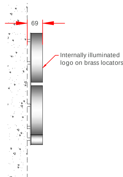
Cross Section Scale 1:10 @A3
