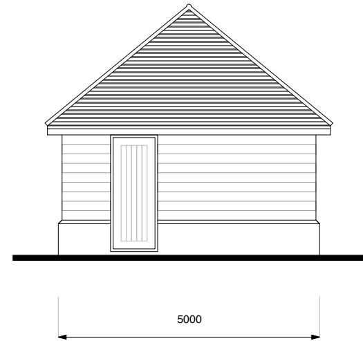
Proposed NORTH WEST (Side) Elevation at 1:100 scale
