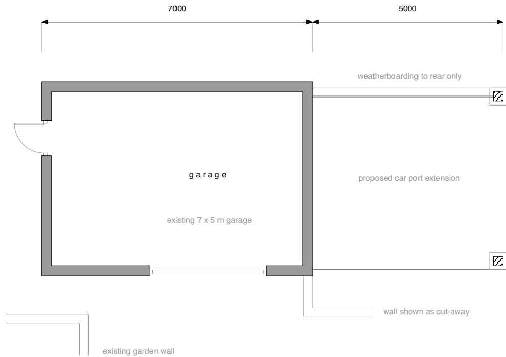
Proposed Floor Plan at 1:100 scale
