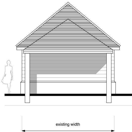
Proposed SOUTH EAST (Side) Elevation at 1:100 scale
