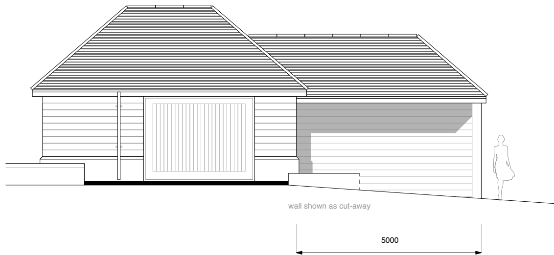
Proposed NORTH EAST (Front) Elevation at 1:100 scale
