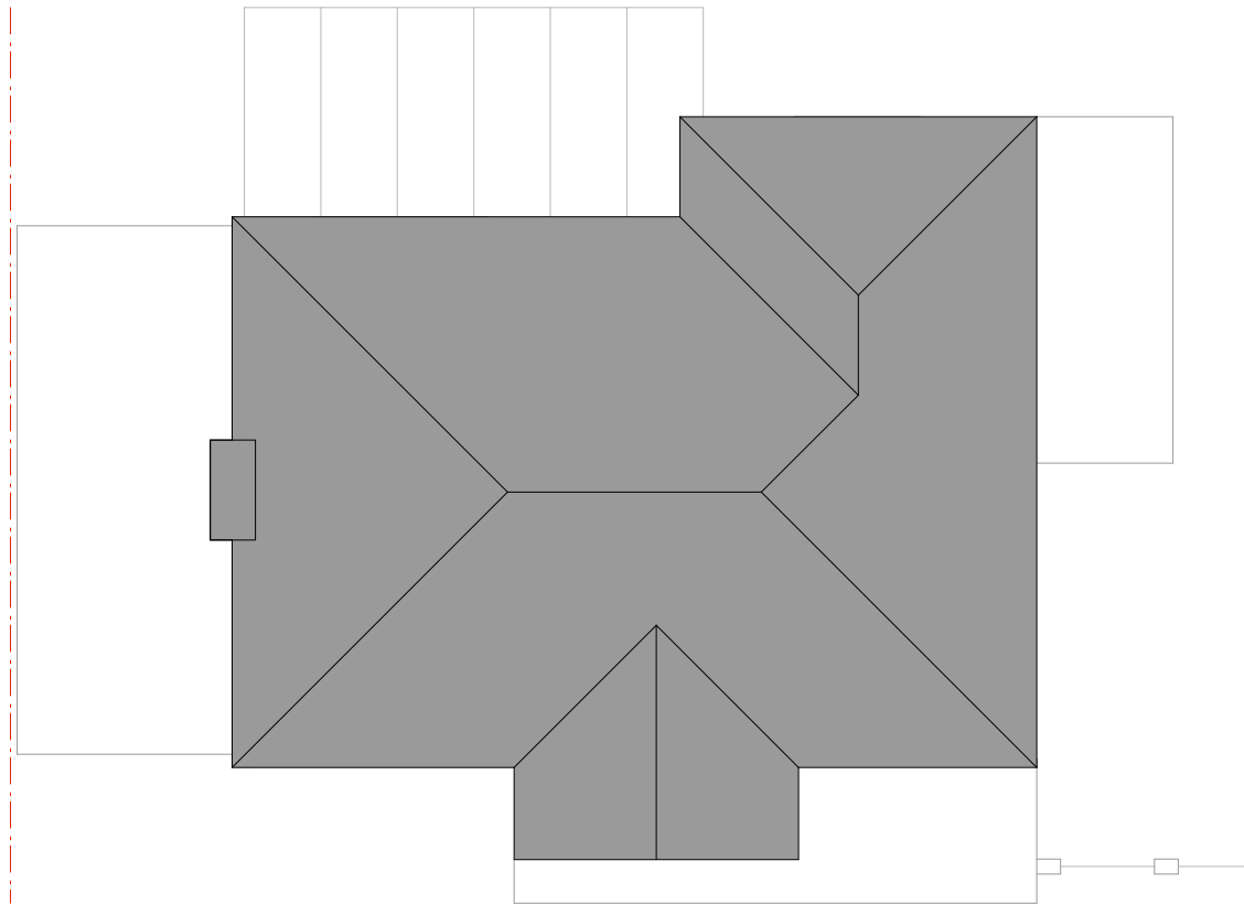
Existing Roof Plan at 1:100 scale
