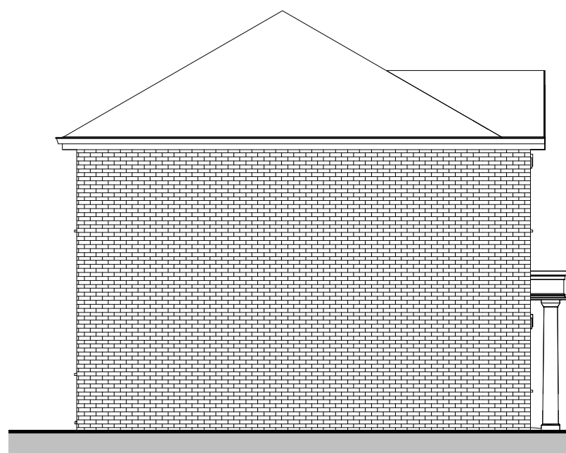
3 East Elevation HT B 1 : 100
