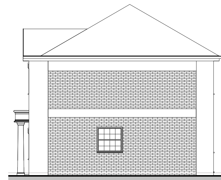
6 West Elevation HT B 1 : 100
