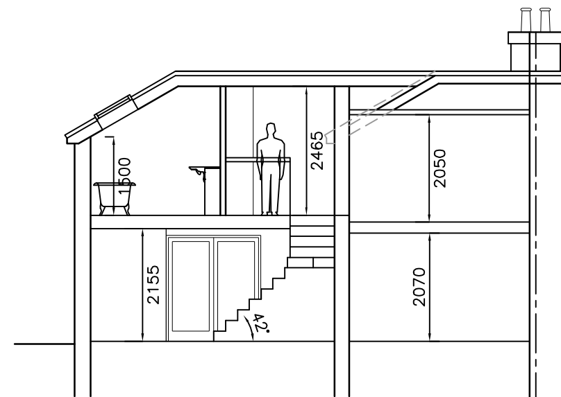
DRAFT SECTION
