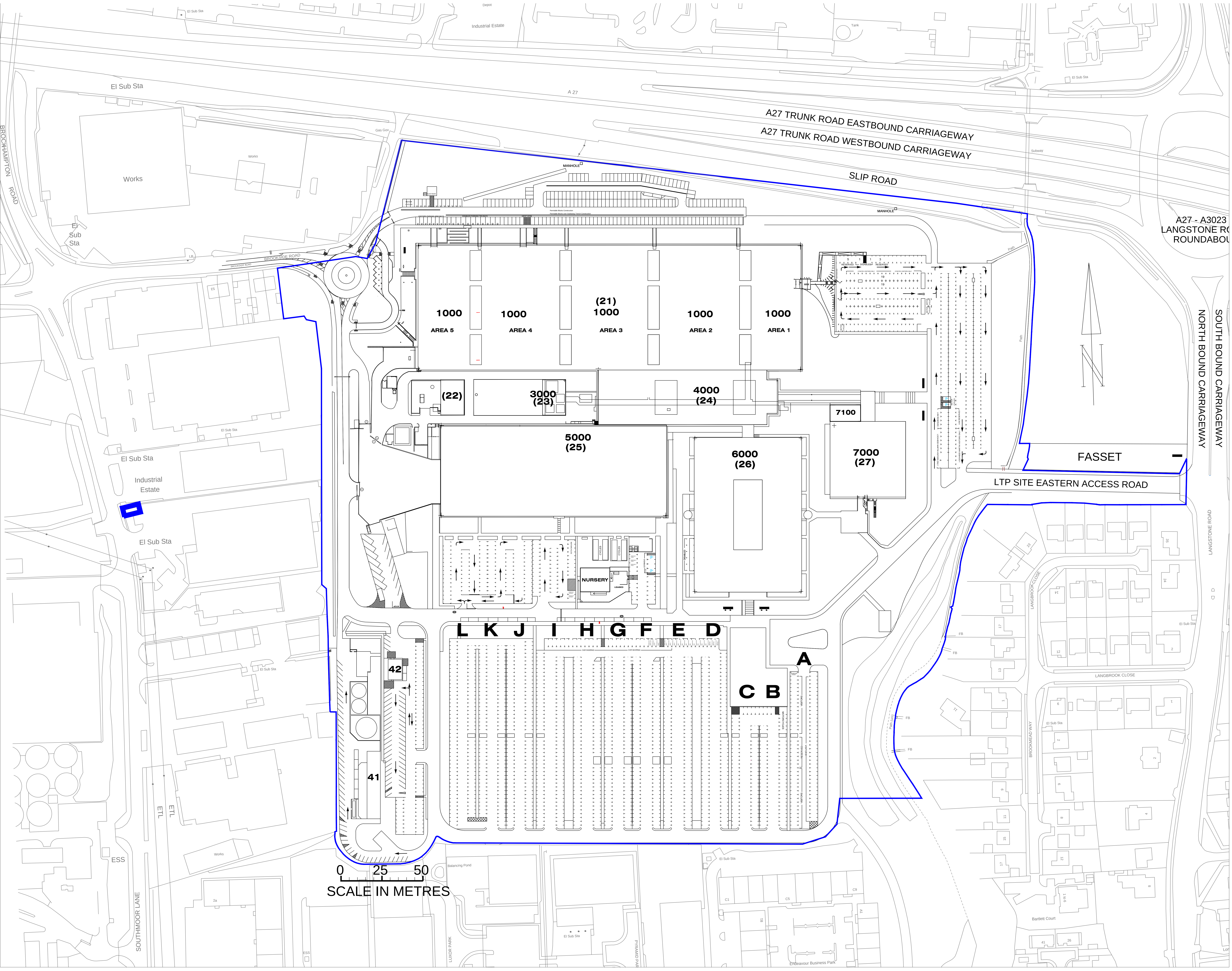
LANGSTONE TECHNOLOGY PARK MPH SITE SCHEMATIC 1:1000
