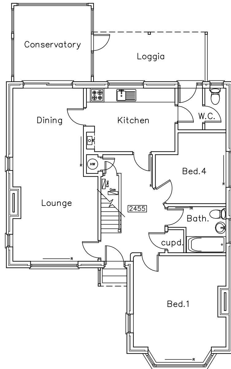
GROUND
