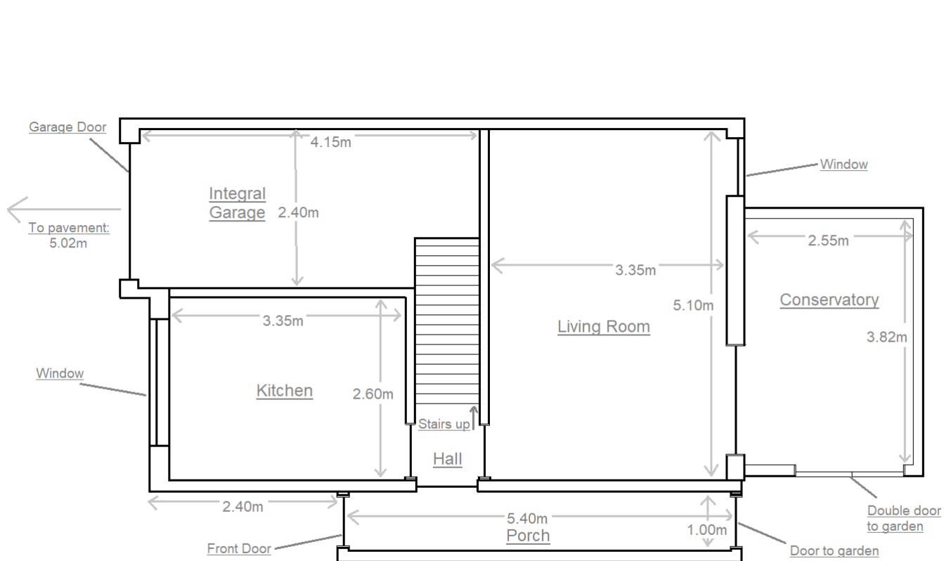
6 Mountbatten Drive Ground Floor Plan - Existing
