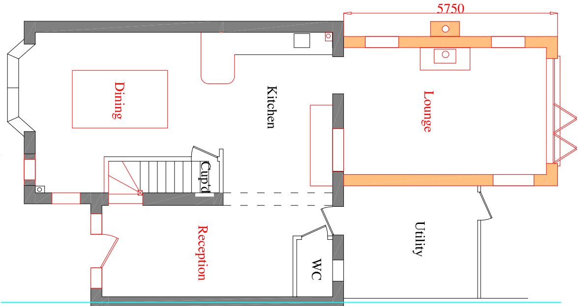
Proposed Ground Floor Layout
