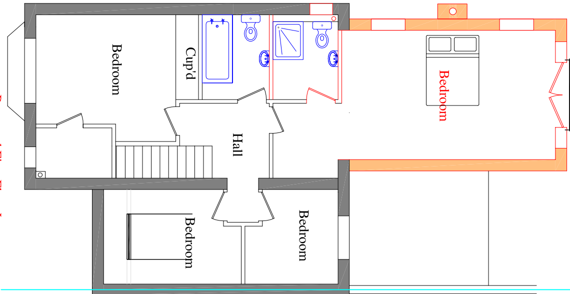
Proposed First Floor Layout
