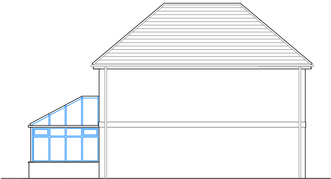
North Elevation
