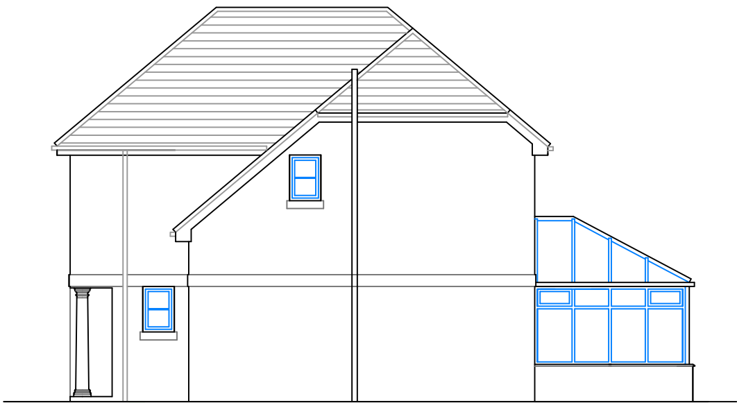
South Elevation
